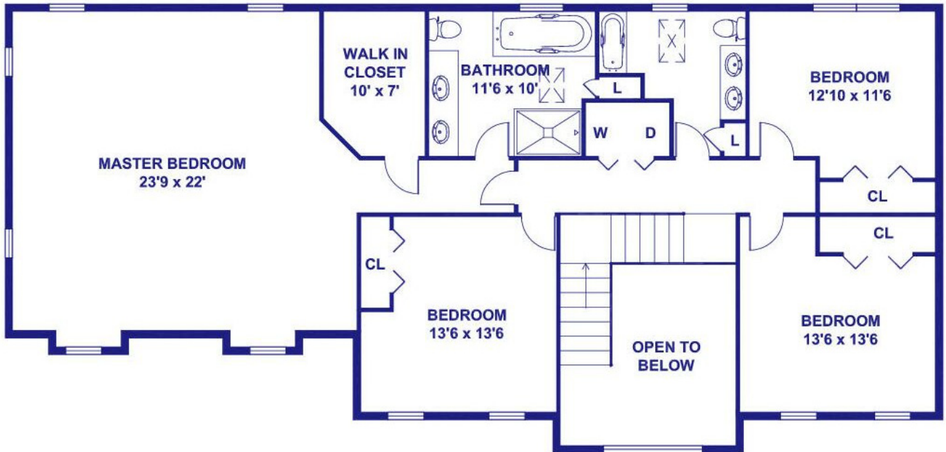
SECOND FLOOR
